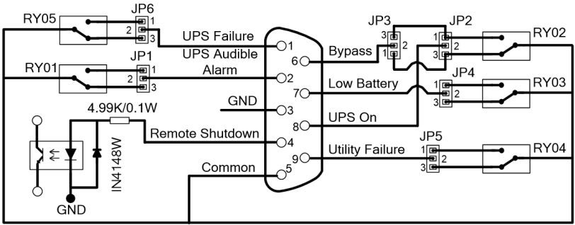
Fig 1 - Pin definition and internal logical connection
